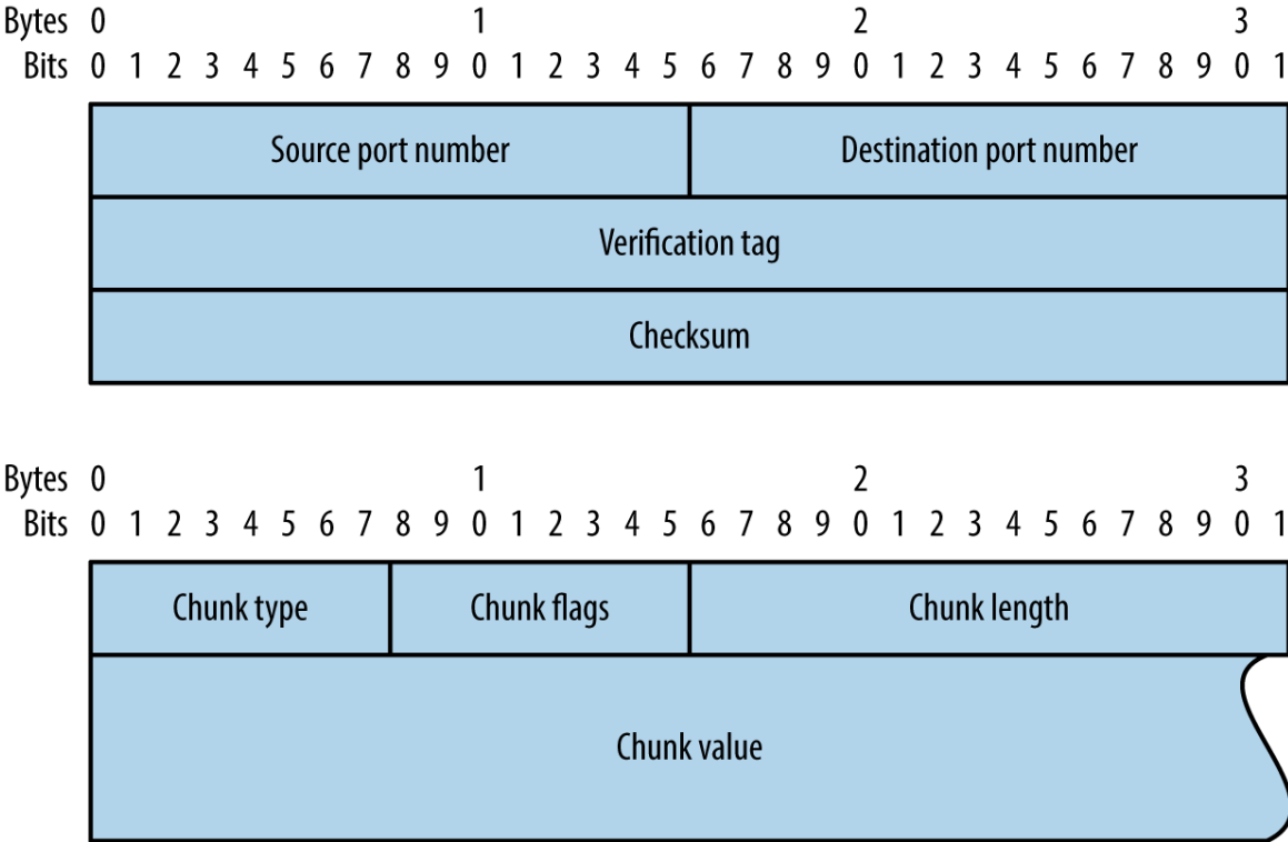
Figure 6-6. SCTP packet format
