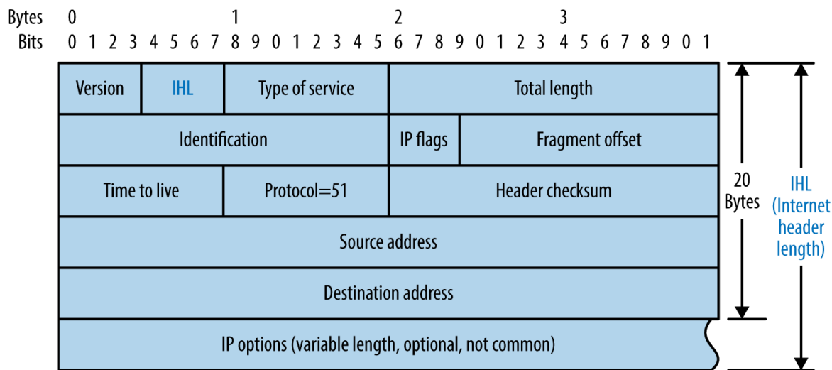
Figure 6-7. IPv4 header format
