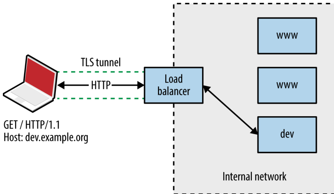
Figure 13-2. Abusing a misconfigured proxy
