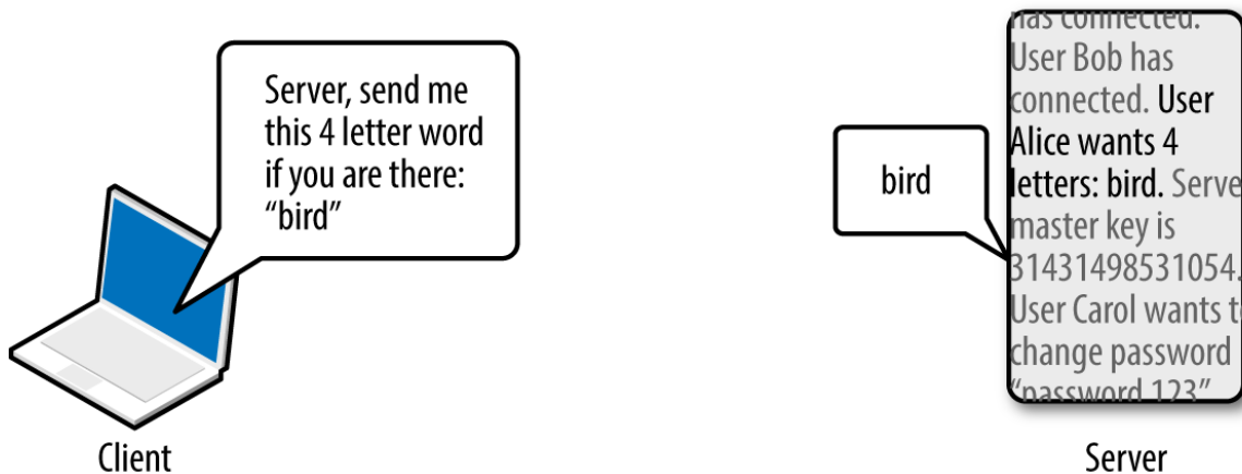
Figure 3-8. A server fulfilling a TLS heartbeat request
