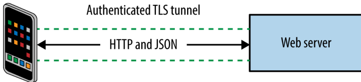
Figure 12-4. Protocols and data formats used by an iOS application
