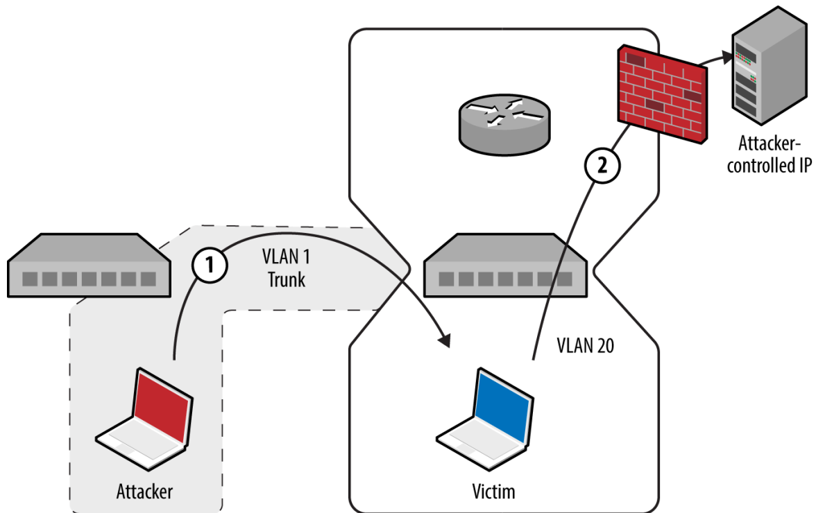
Figure 5-7. Bypassing security controls by double-tagging
