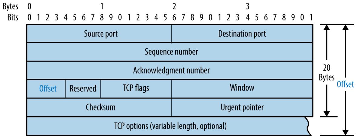
Figure 6-8. TCP header format
