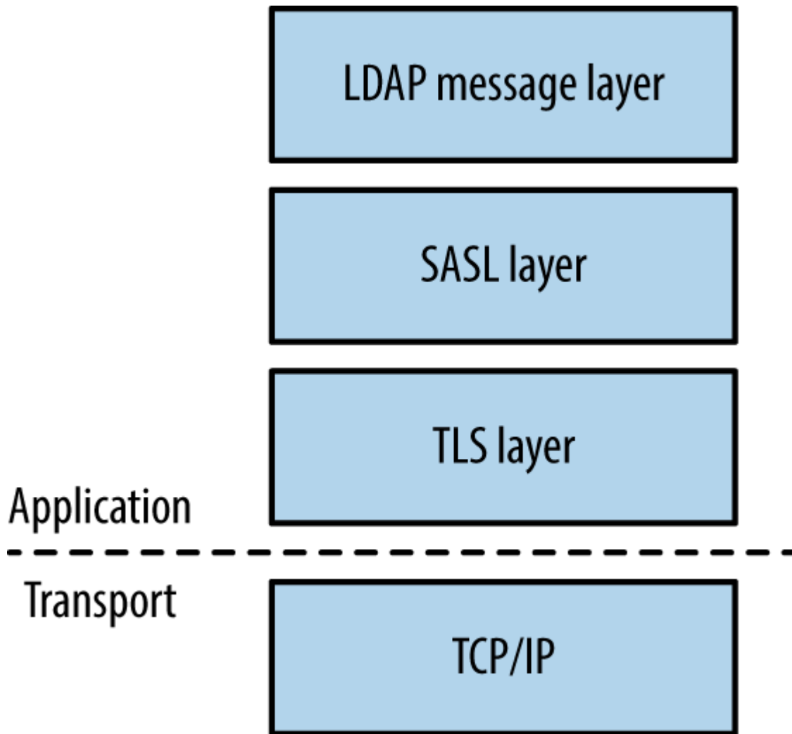
Figure 7-3. LDAP layers when using TLS
