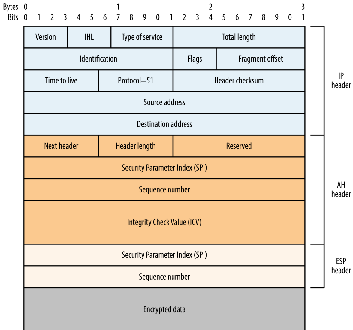
Figure 10-2. IPsec datagram format (tunnel mode)
