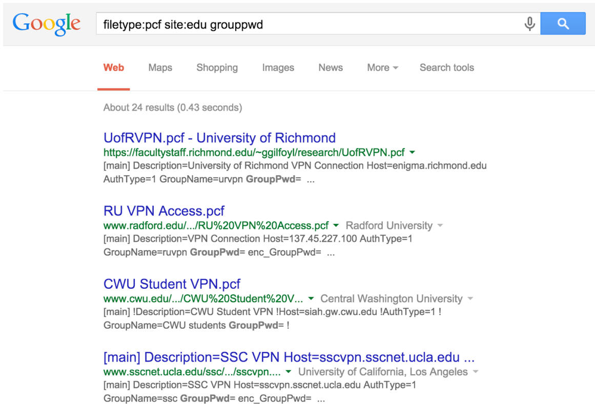
Figure 4-4. Identifying Cisco PCF files via Google
