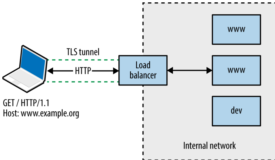
Figure 13-1. Connecting to a virtual host via HTTP 1.1 and TLS
