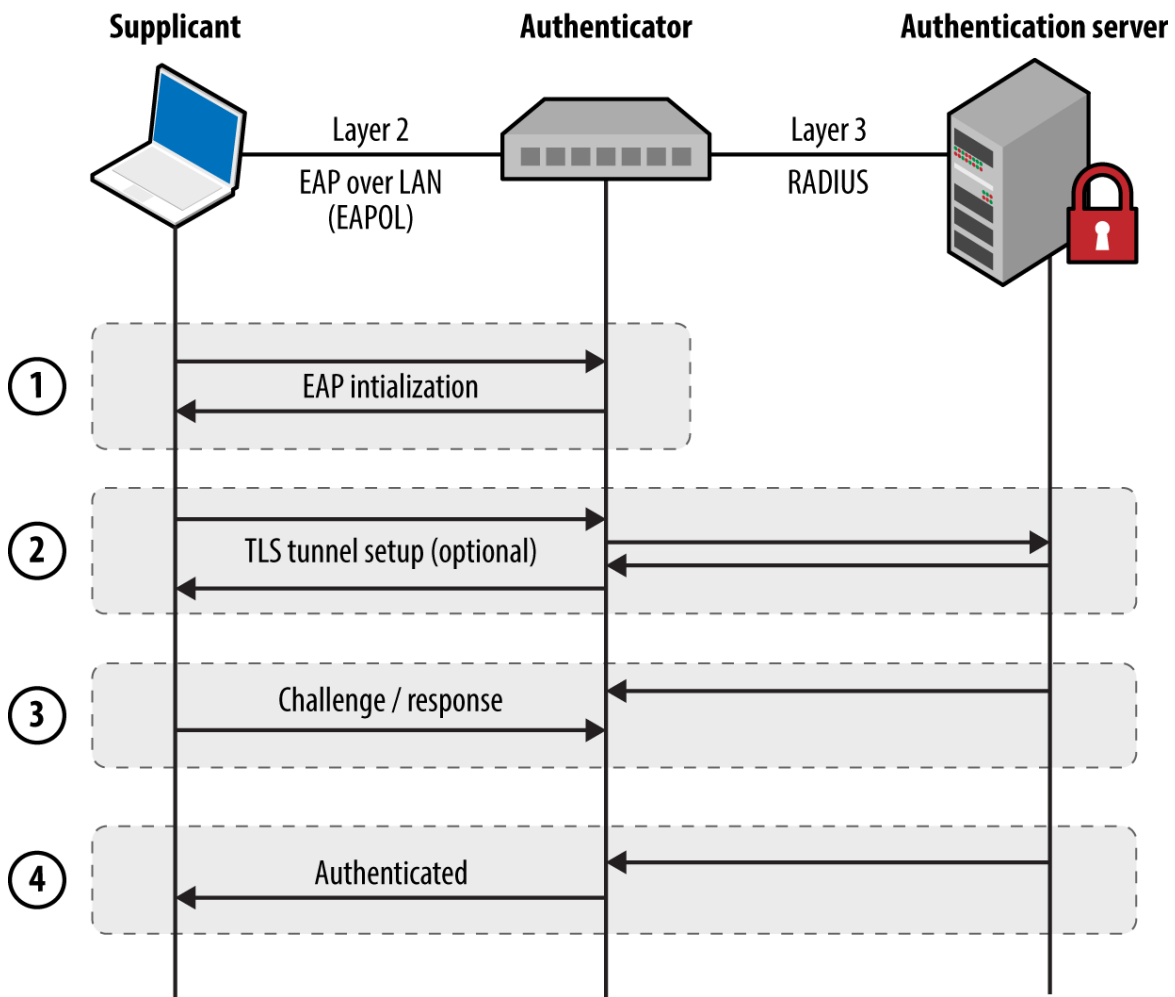
Figure 5-9. 802.1X authentication
