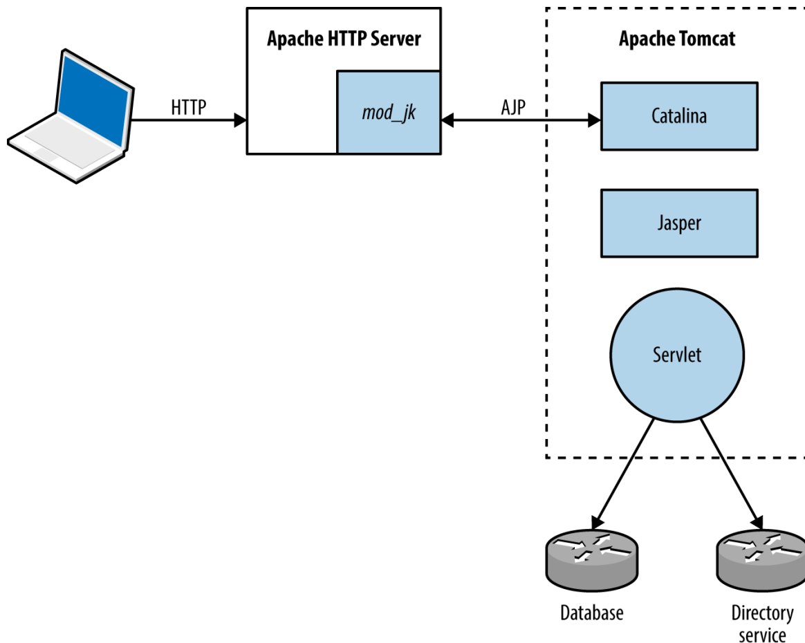
Figure 12-6. The Apache mod_jk connector in-use
