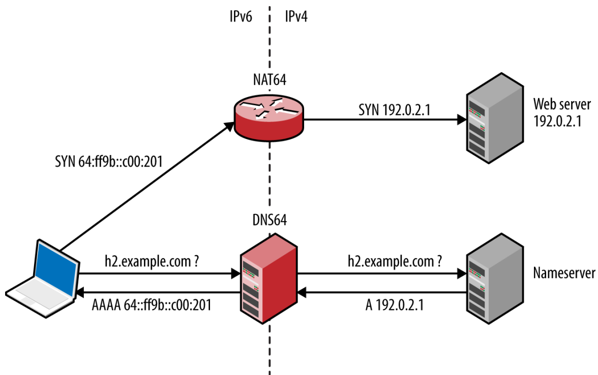
Figure 5-21. Serving IPv6 clients via NAT64 and DNS64
