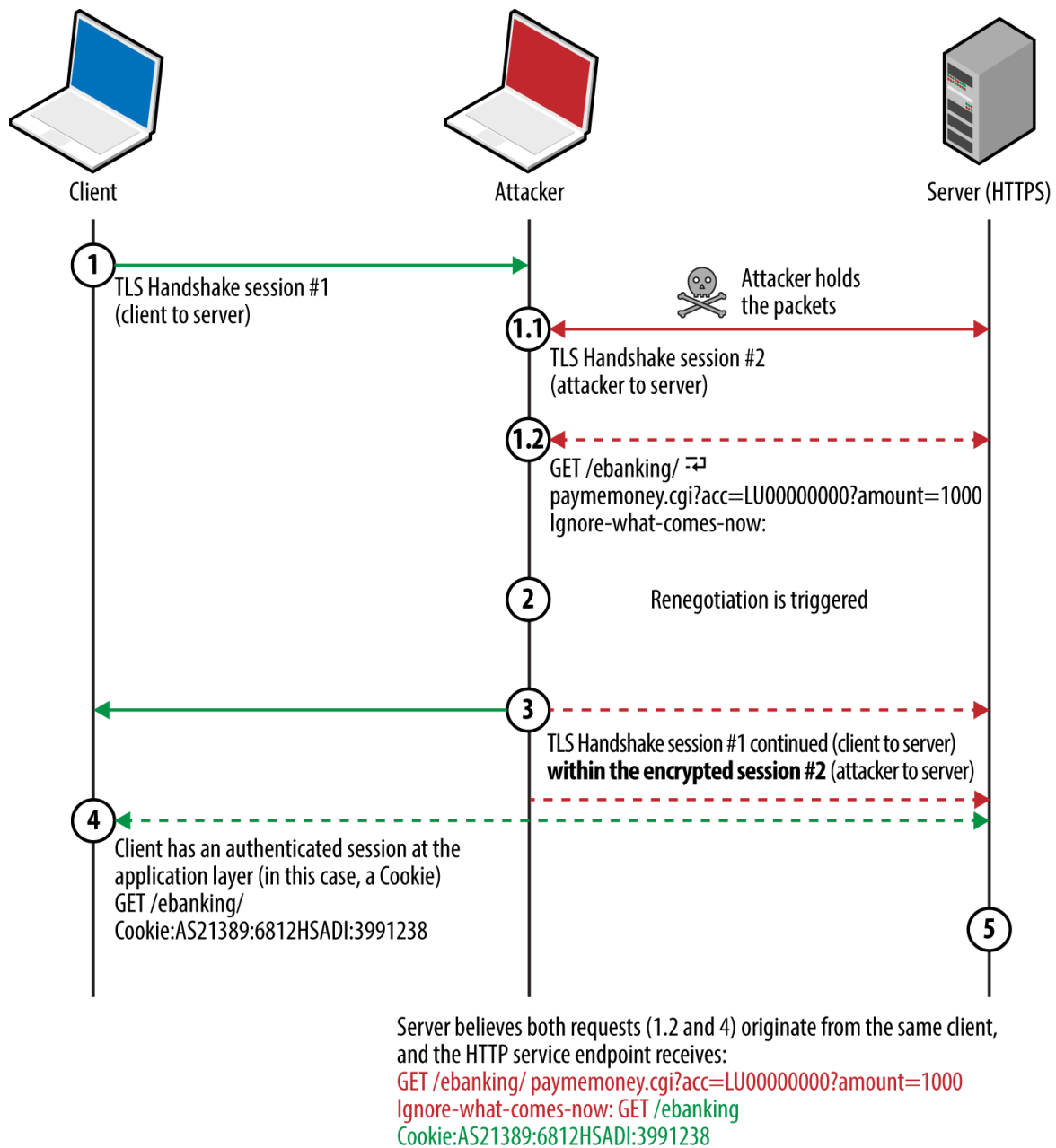
Figure 11-8. HTTPS injection via insecure renegotiation
