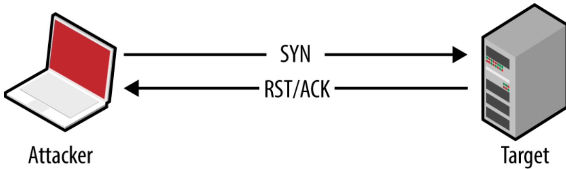
Figure 6-3. Closed port behavior
