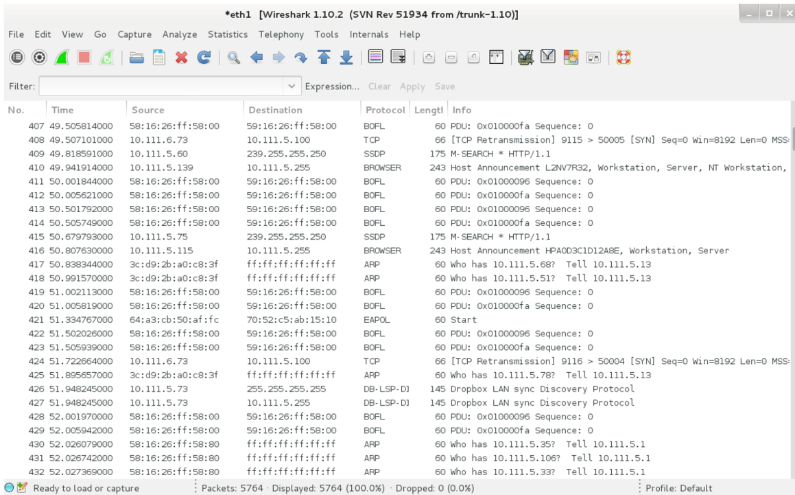
Figure 5-2. Wireshark used to sniff local traffic
