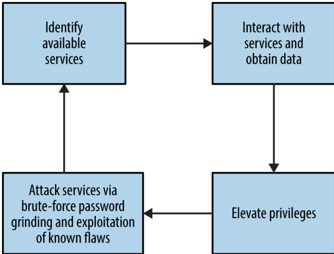
Figure 8-4. Iterative testing of SMB and RPC services
