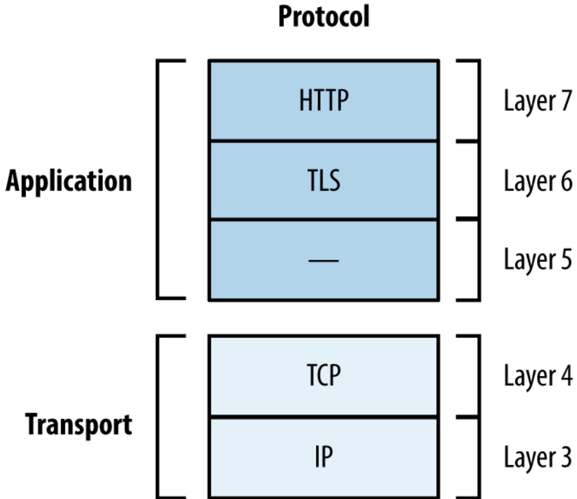
Figure 11-1. TLS belongs to Layer 6
