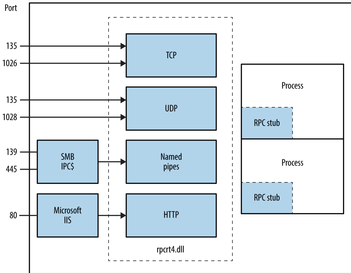
Figure 8-3. Microsoft RPC transport protocols
