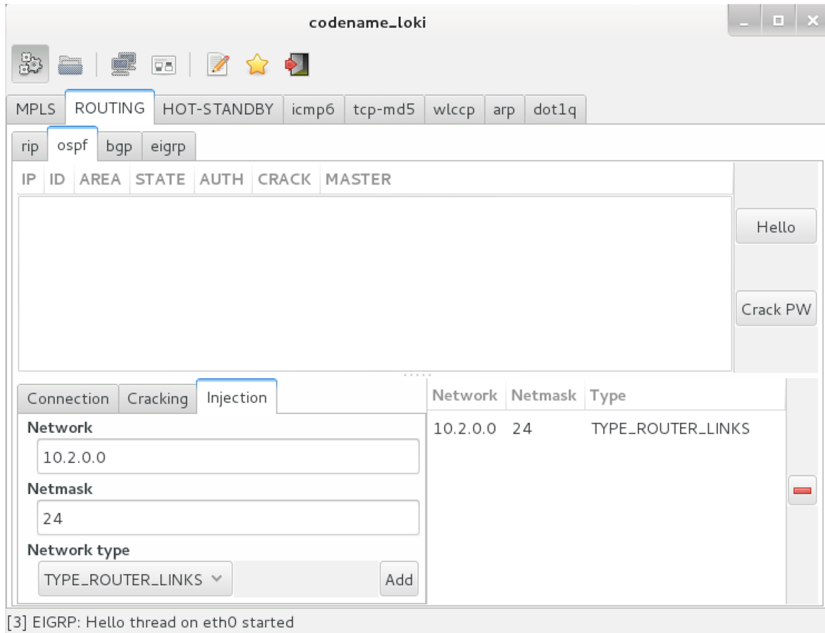
Figure 5-17. Advertising a new OSPF route using Loki
