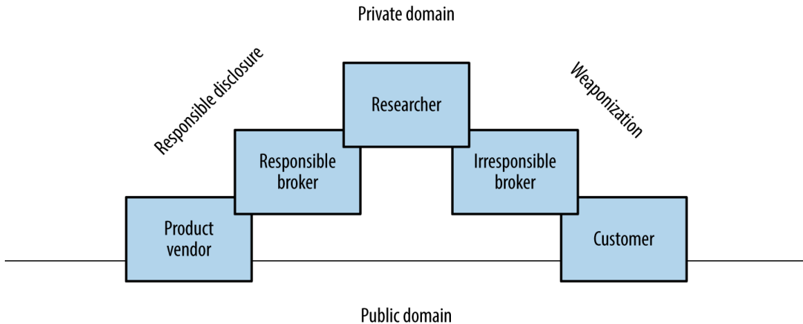
Figure 2-1. Common proliferation paths for vulnerability details
