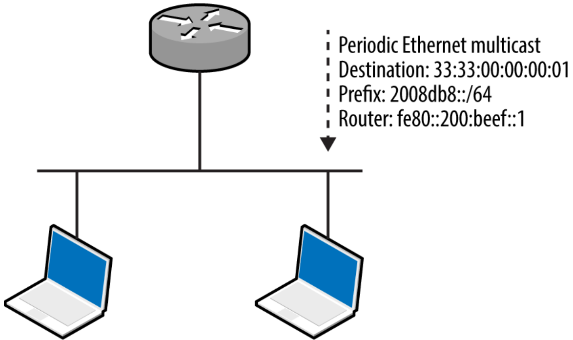
Figure 5-18. IPv6 router advertisement
