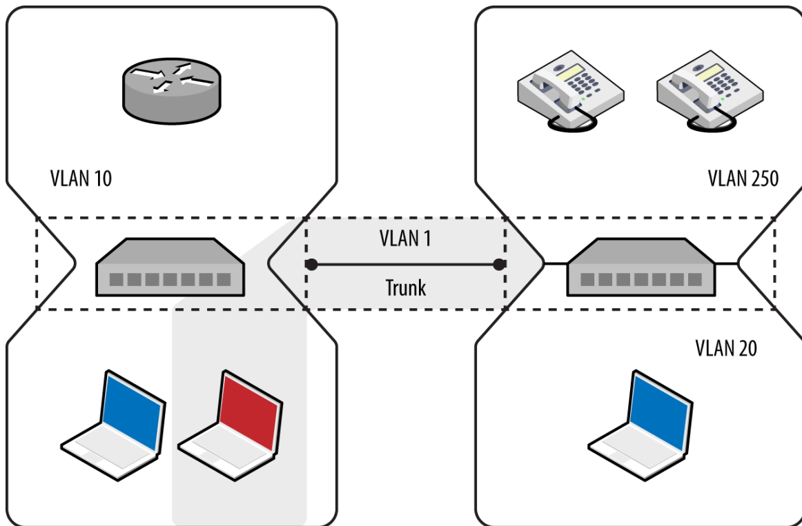
Figure 5-5. Using DTP to enable trunking on a local port
