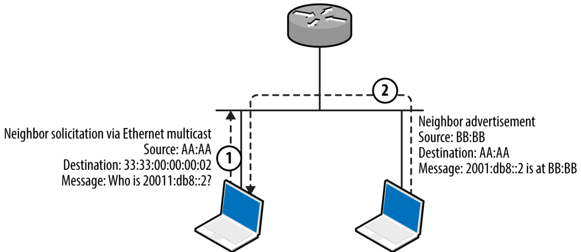
Figure 5-19. IPv6 neighbor solicitation and advertisement
