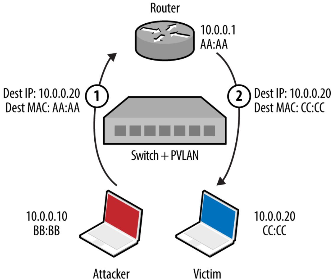
Figure 5-8. A private VLAN attack
