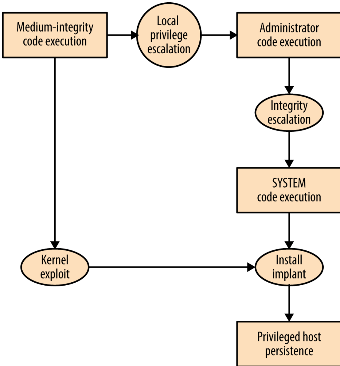
Figure 3-5. Local privilege escalation attack graph
