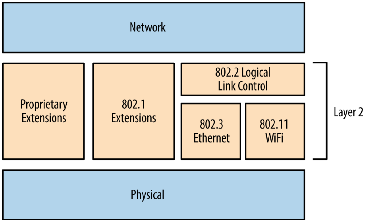
Figure 5-1. The physical, data link, and network layers
