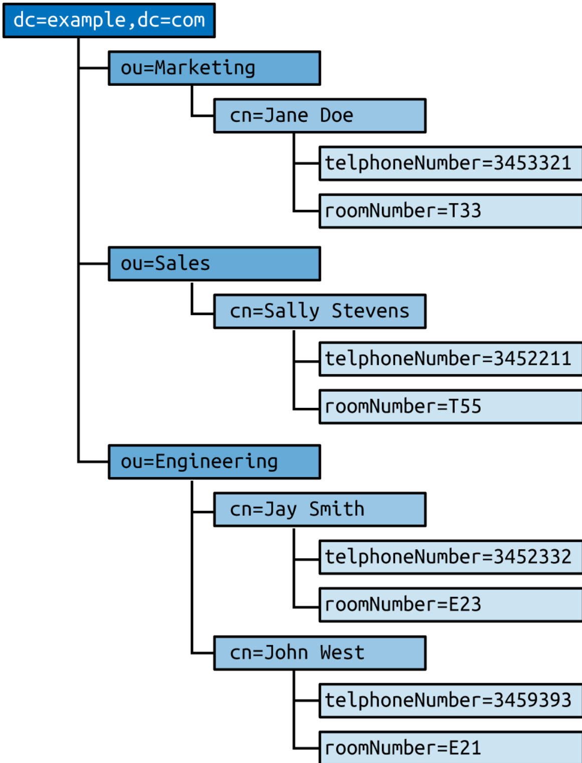
Figure 7-4. An LDAP directory structure
