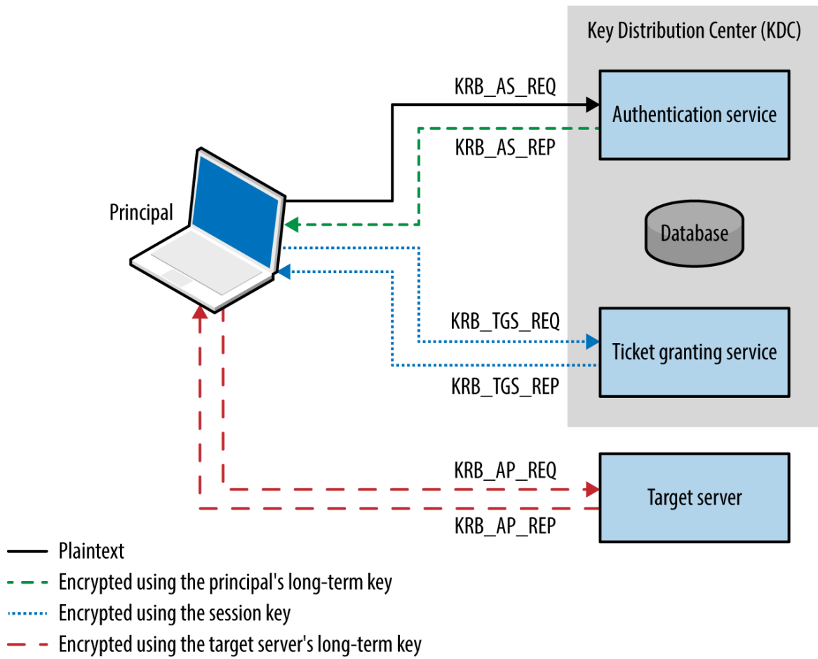
Figure 7-5. Kerberos KDC authentication and ticketing
