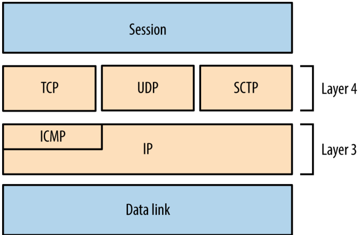
Figure 6-1. Network protocols and respective OSI layers
