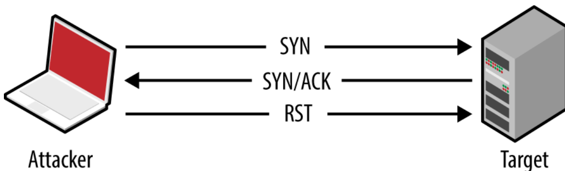
Figure 6-2. Open port behavior
