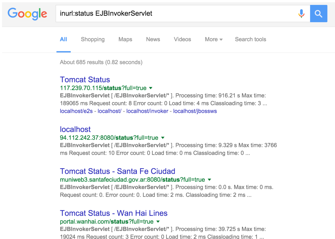
Figure 14-7. Using Google to find exposed JBoss invoker servlets
