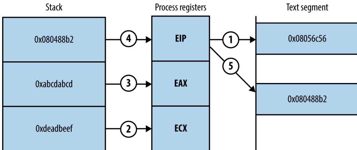
Figure 3-10. Prepared stack frame and CPU register values
