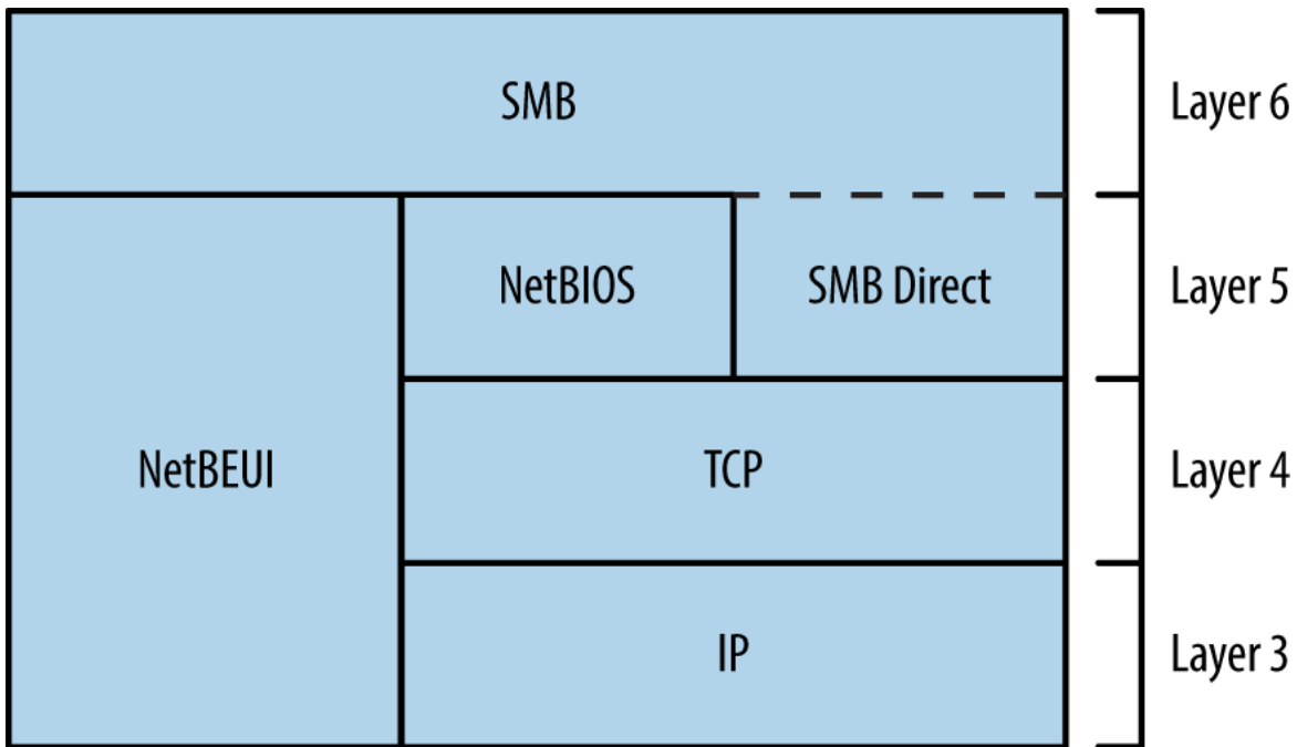
Figure 8-2. SMB is available through different services
