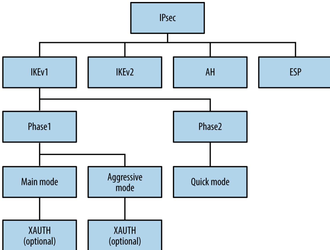
Figure 10-3. IPsec protocol components
