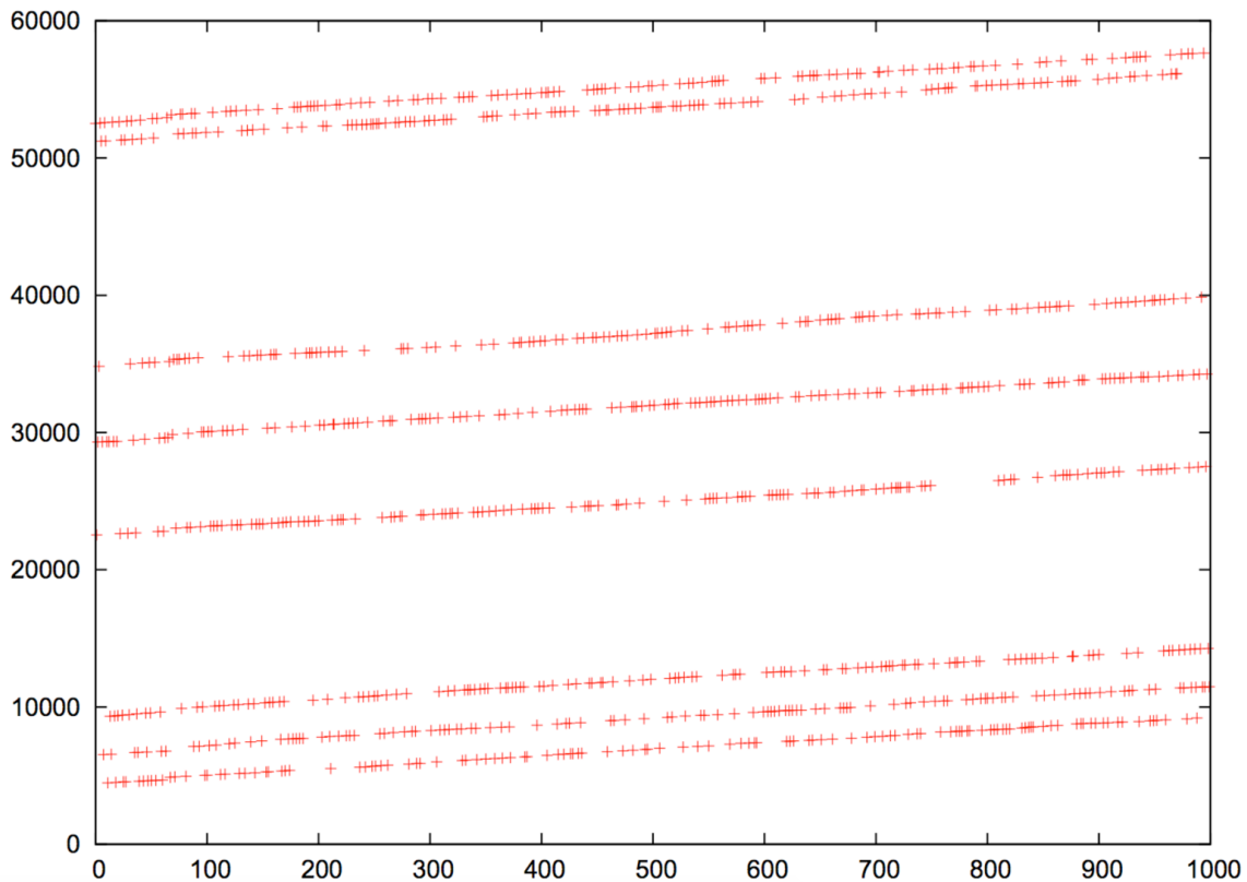
Figure 6-9. IP ID value plot for www.yahoo.fr
