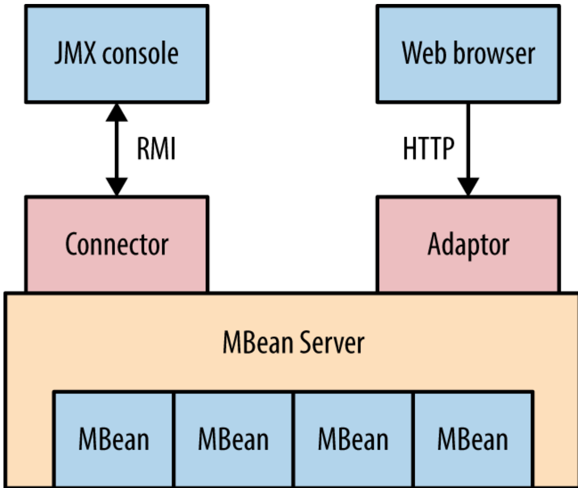
Figure 14-4. JBoss architecture and components
