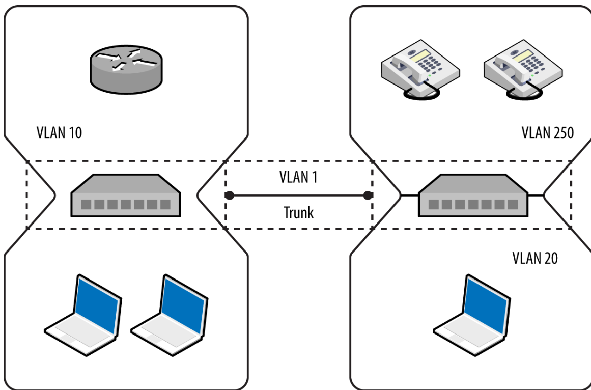
Figure 5-4. A typical network using 802.1Q VLAN tagging
