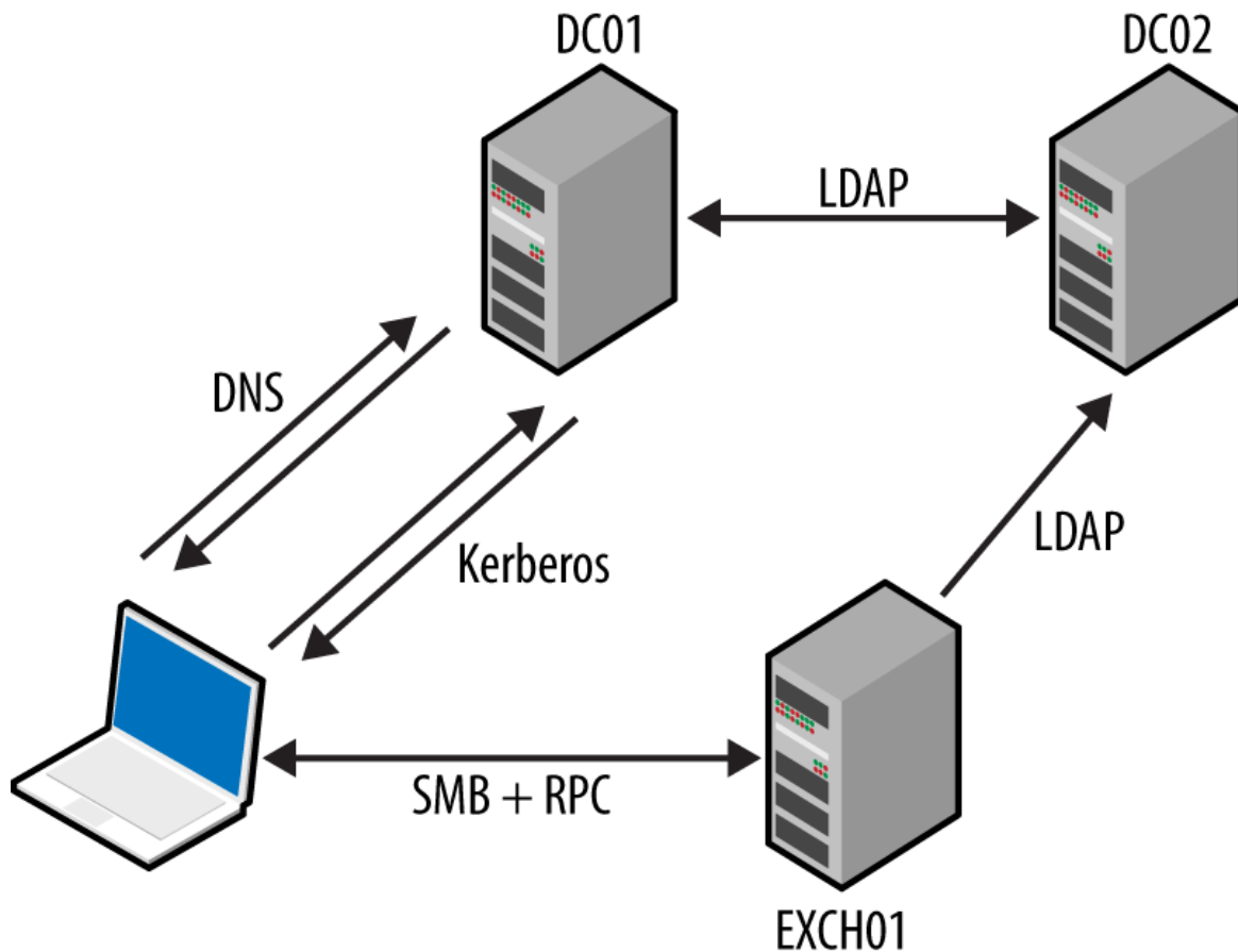
Figure 8-1. Protocols supporting Microsoft Exchange and Outlook
