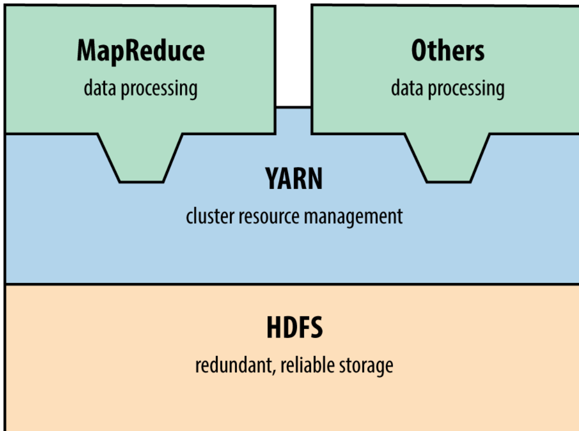
Figure 15-1. Hadoop 2.0 architecture
