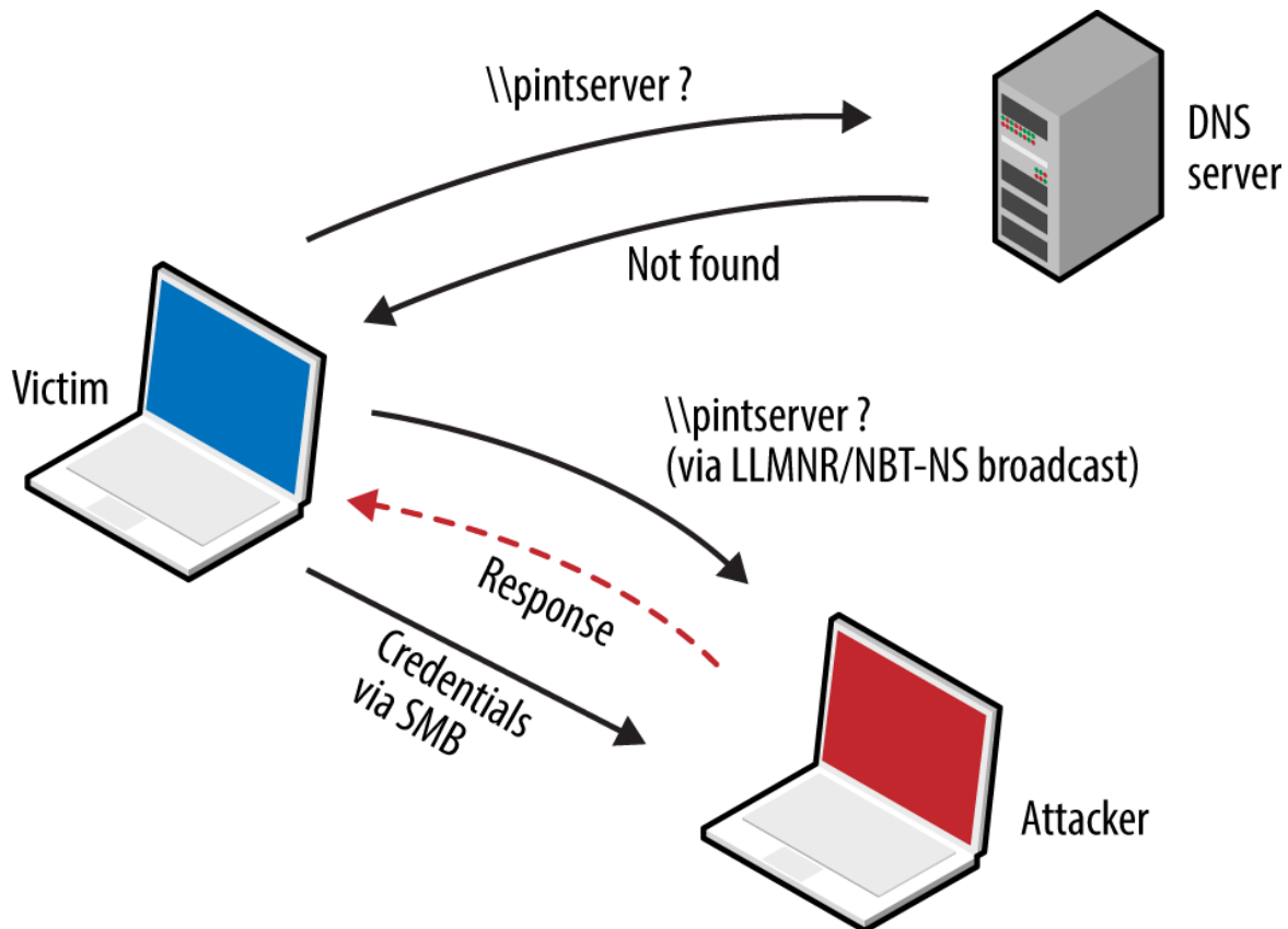
Figure 5-14. LLMNR/NBT-NS poisoning
