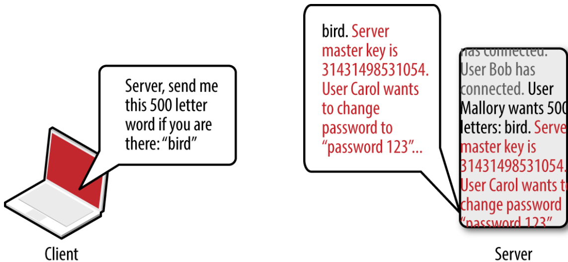
Figure 3-9. A malicious TLS heartbeat request revealing heap content
