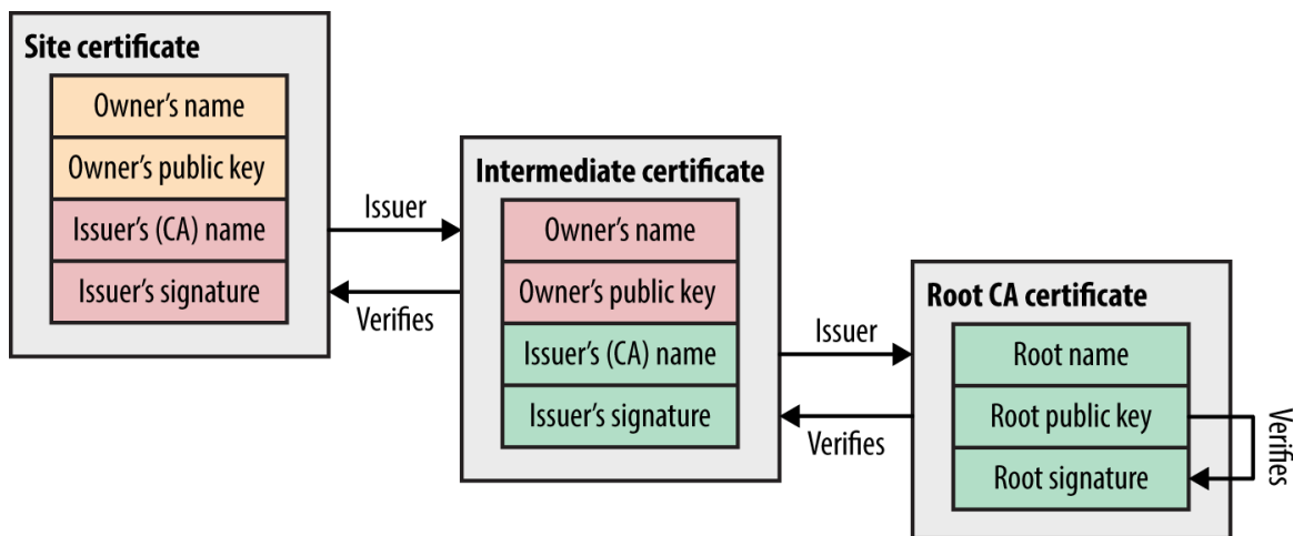
Figure 11-6. An X.509 certificate chain
