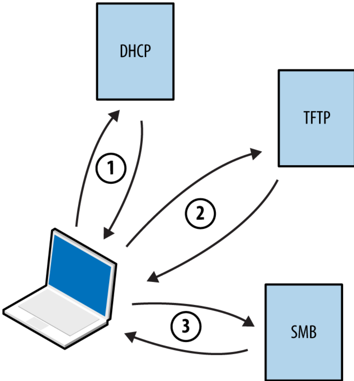
Figure 5-13. Microsoft PXE boot sequence
