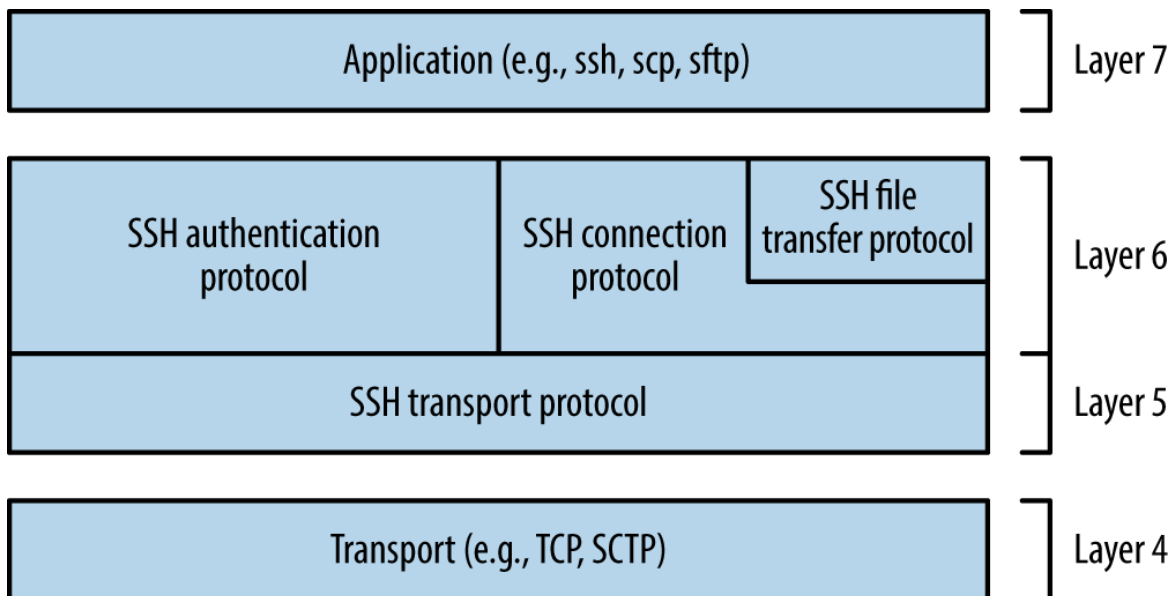
Figure 7-1. SSH 2.0 architecture
