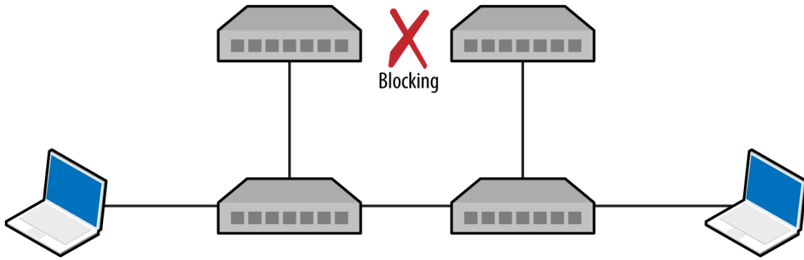
Figure 5-11. An 802.3 Ethernet network using STP
